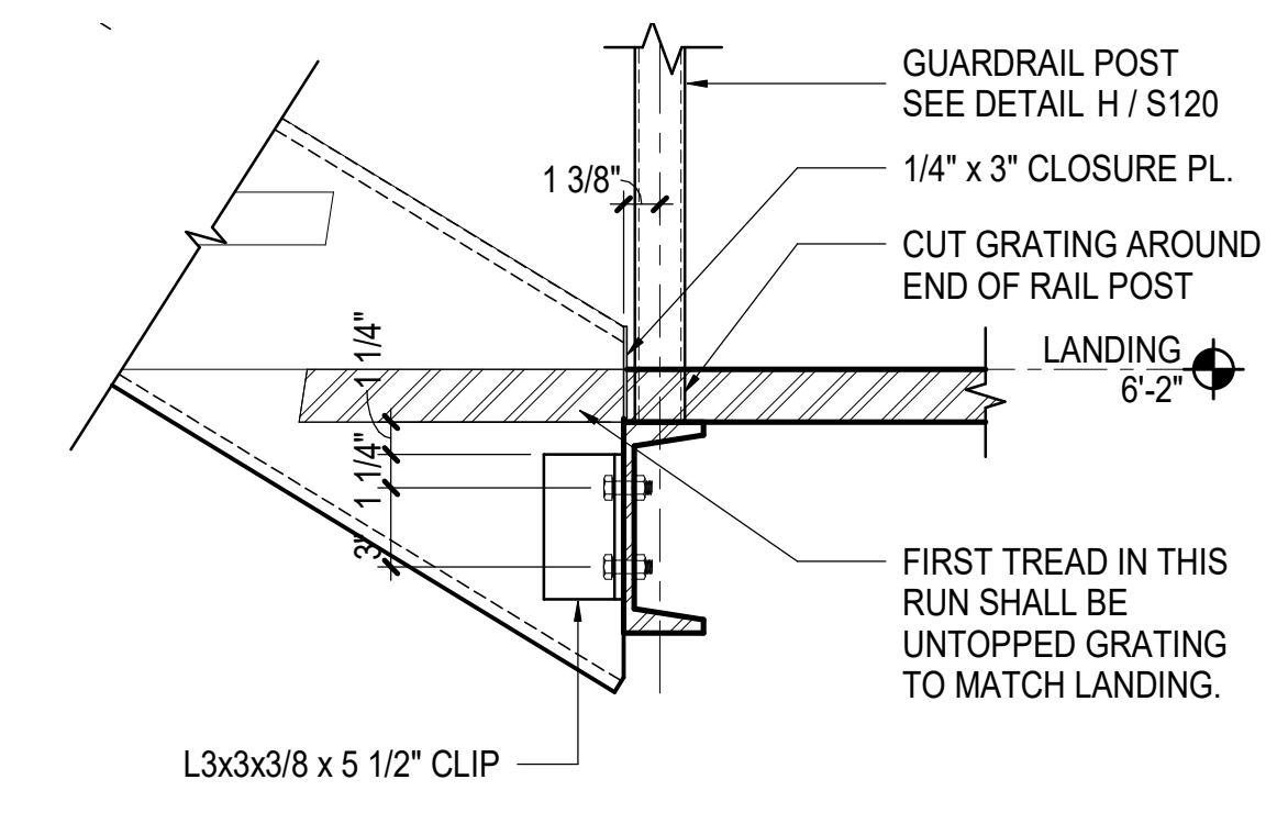
(E) STAIR LANDING BACK CONN. DETAIL 1 1/2" = 1'-0"
