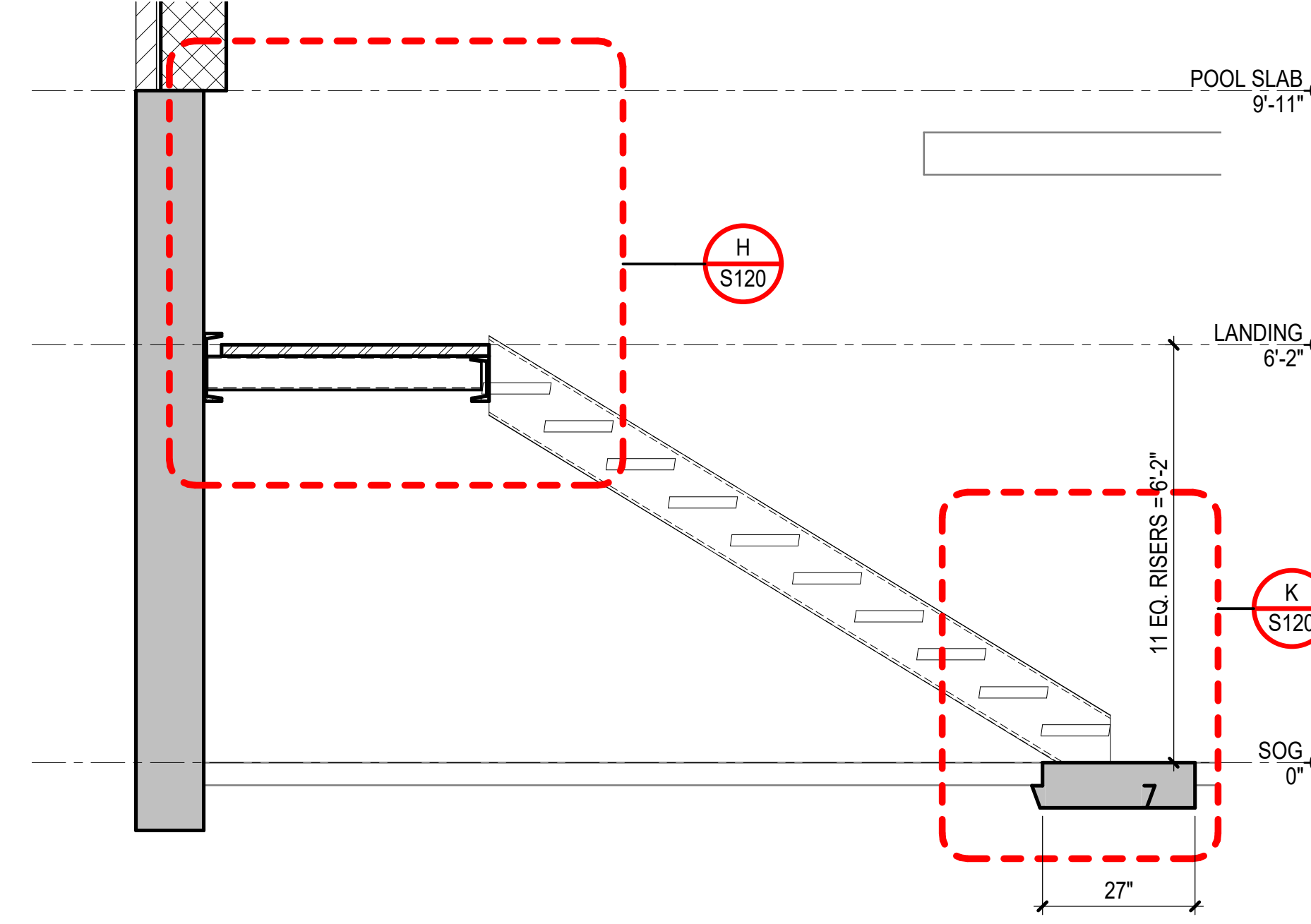
(B) STAIR ELEVATION DETAIL 1/2" = 1'-0"
