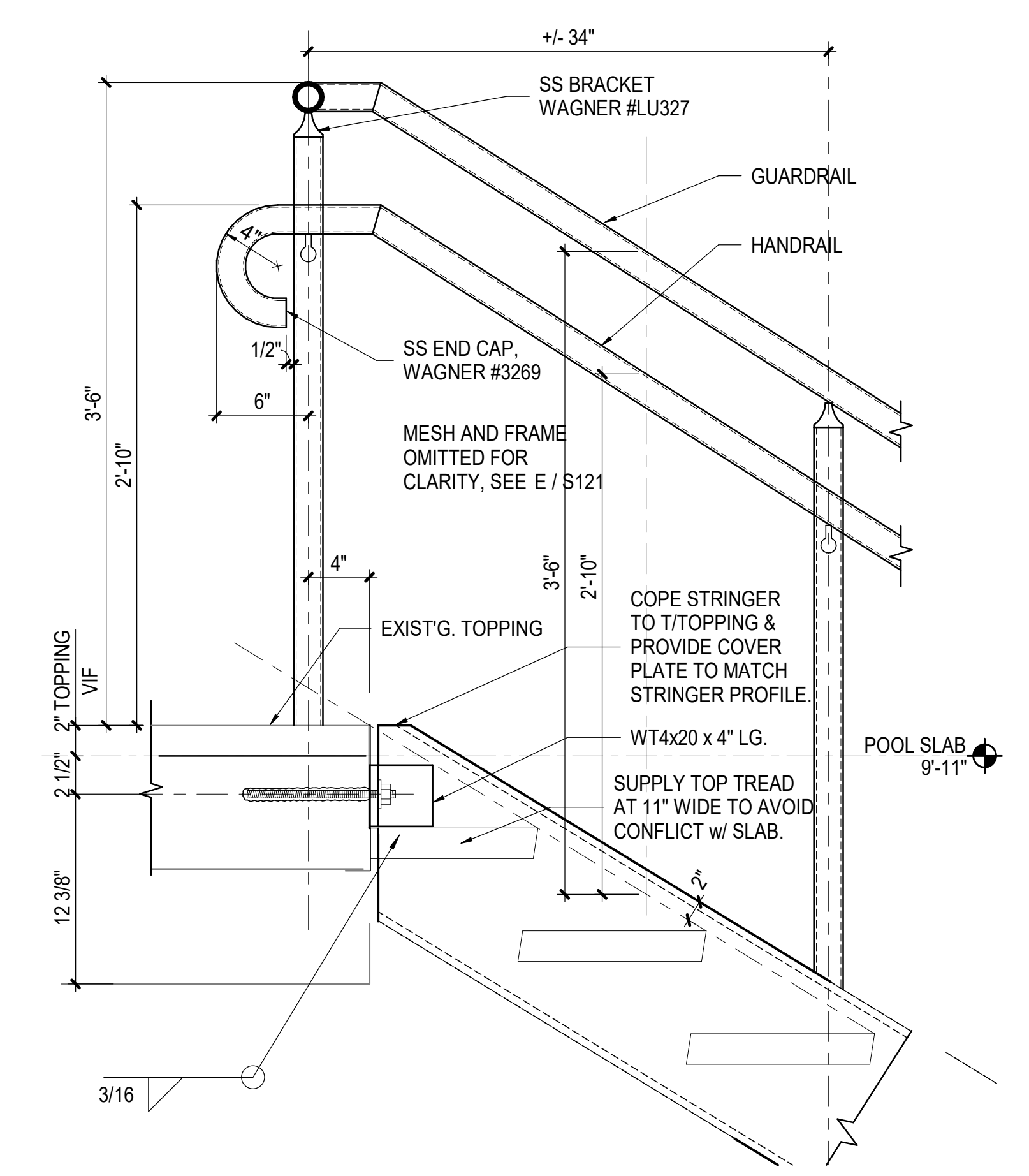
(L) STRINGER CONN. TO DECK SLAB 1 1/2" = 1'-0"
