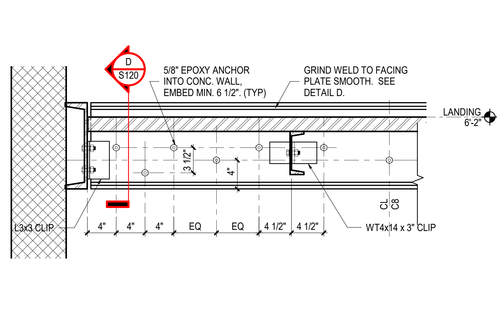
(E) STAIR LANDING BACK CONN. DETAIL 1 1/2" = 1'-0"
