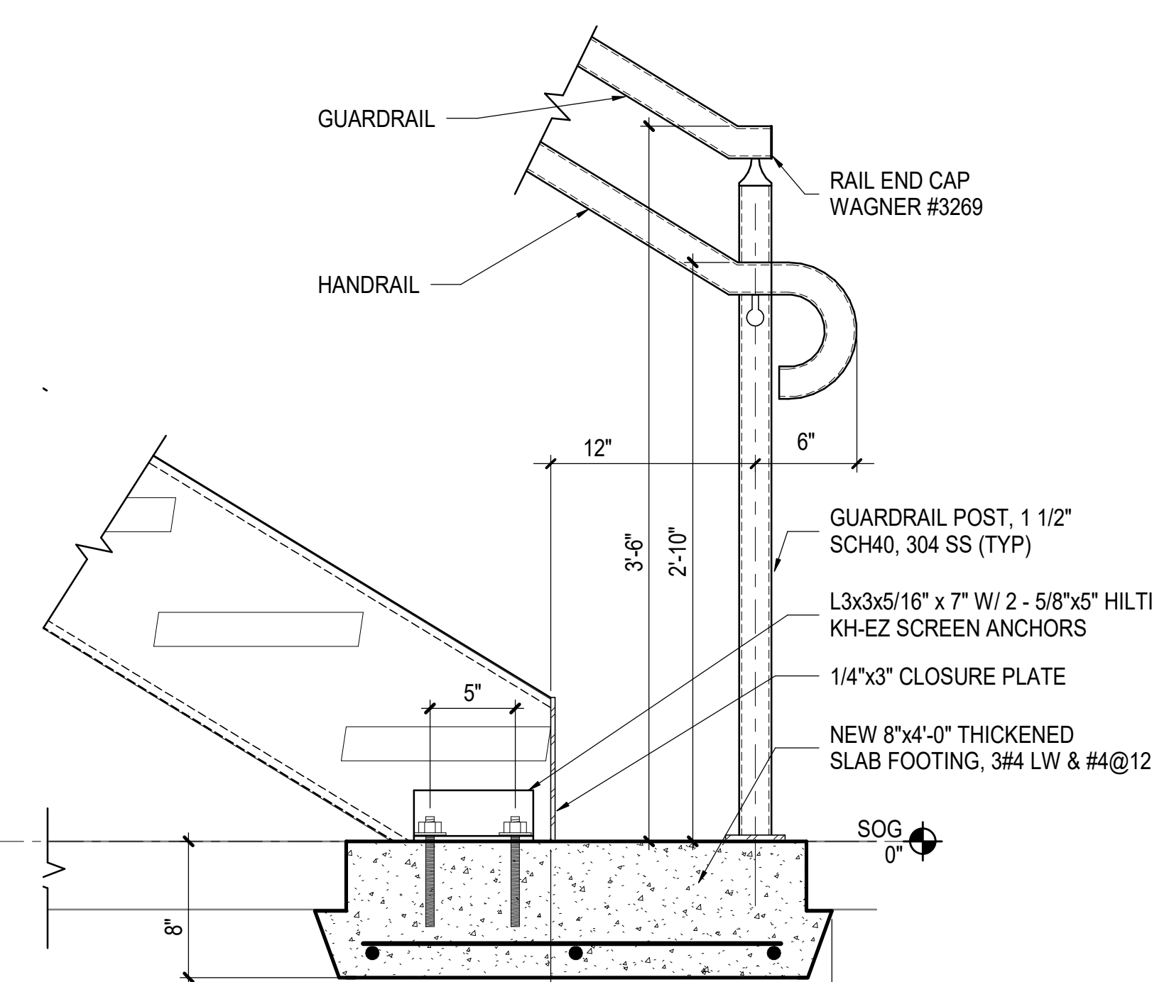
(K) STRINGER BASE CONN. DETAIL 1 1/2" = 1'-0"
