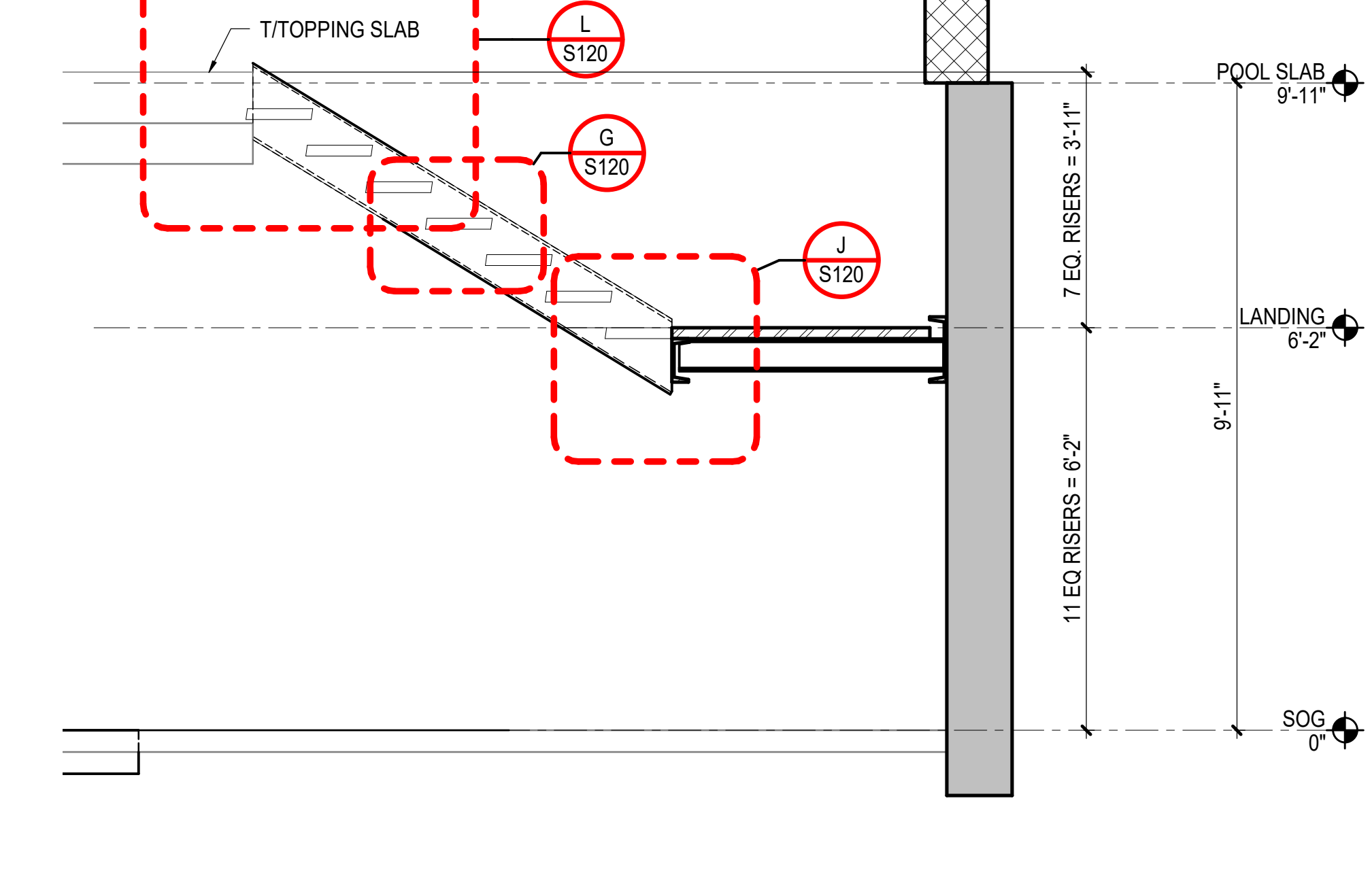
(C) STAIR ELEVATION DETAIL 1/2" = 1'-0"
