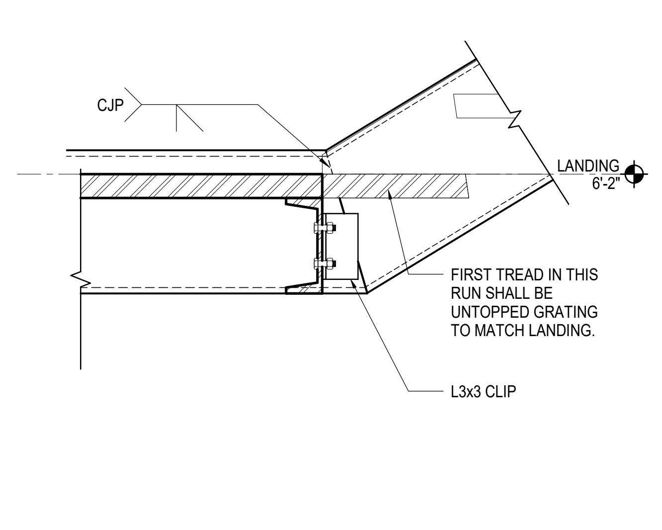
(F) STAIR LANDING HIGH STRINGER CONN. 1 1/2" = 1'-0"
