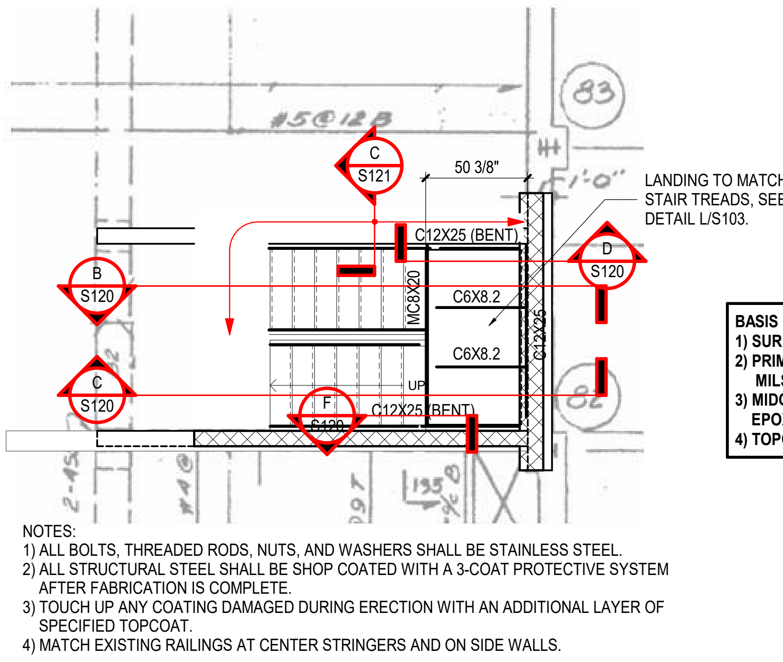
(A) NEW STAIR FRAMING REFERENCE PLAN 1 1/2" = 1'-0"
