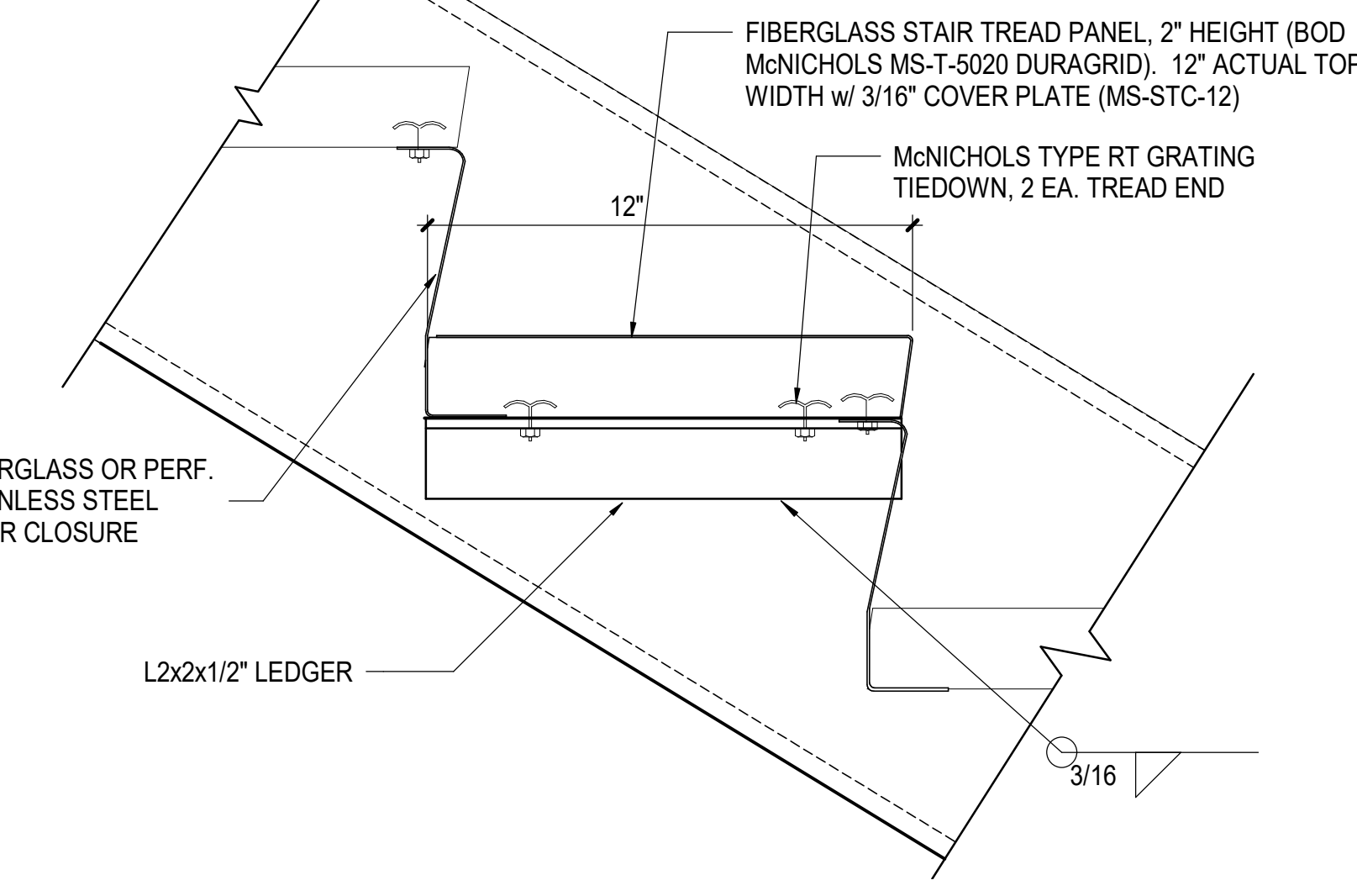
(G) STAIR TREAD CONN. DETAIL 3\"/>
